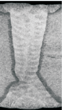
Sectional view of a milled weld seam
